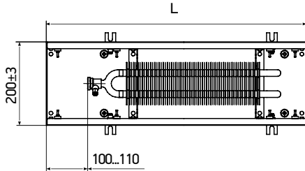
KVZ 200-140
