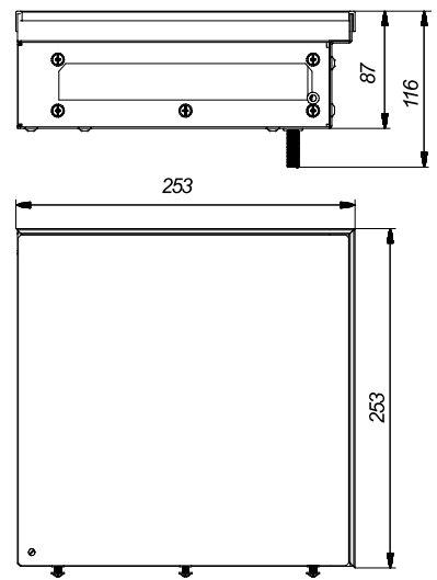
KVU 250-105-135
