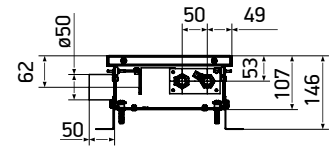
KVVZ 250-105
